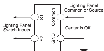
KSW-T
