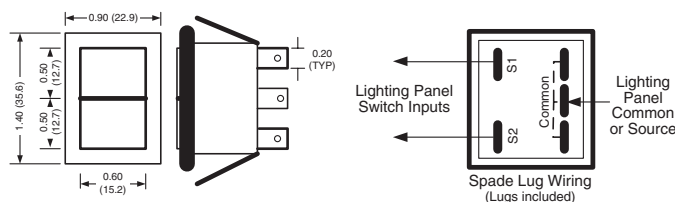
KSW-P2
